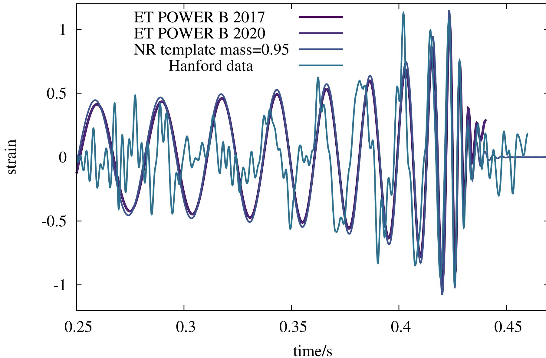
Strain GW150915: ET-2020-05, NR template and Hanford data
